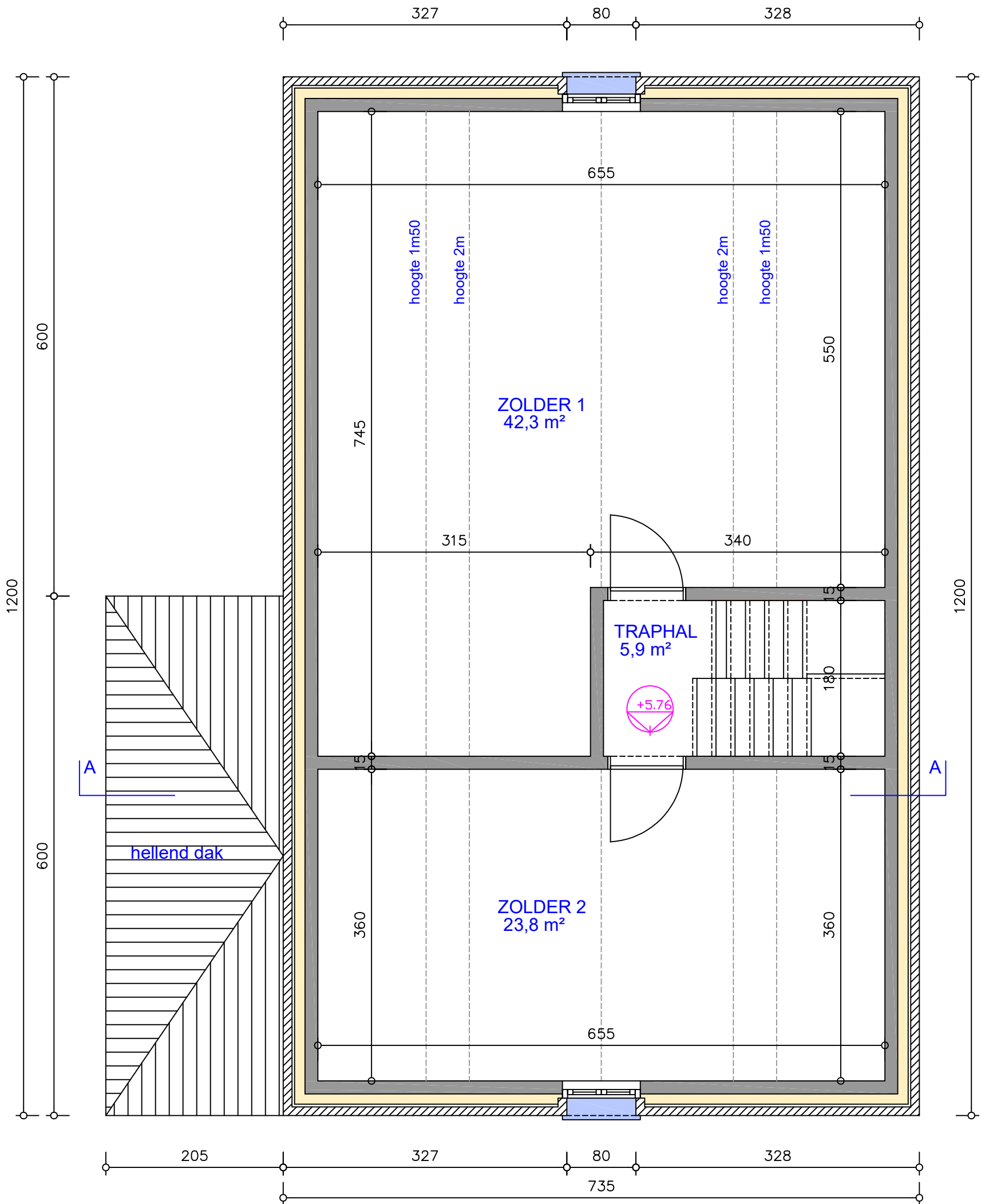
PLAN ZOLDER
